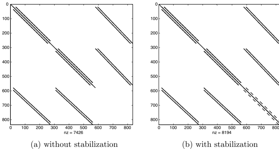
Figure 2.1. Sparsity patterns for two-dimensional Stokes problem (leaky lid-driven cavity) using Q1-P0 discretization.
