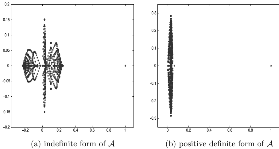
Figure 3.1. Eigenvalues for two-dimensional Oseen problem (leaky lid-driven cavity) using Q1-P0 discretization.
